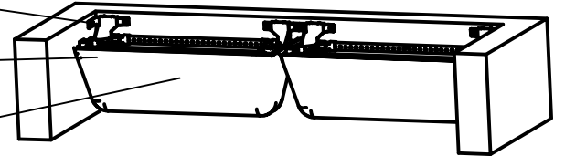
FLEXSTORM HDWM WALL MOUNT INLET FILTERS FOR OPEN THROAT GUTTERS (2 piece set for 6', 7', 8')
